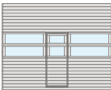
DOOR WITH PASS-THROUGH DOOR, PANELS WITH ALUMINIUM GLAZED SECTION
