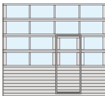
DOOR WITH PASS-THROUGH DOOR, PANELS WITH ALUMINIUM GLAZED SECTION
